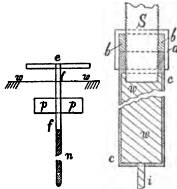
FIG. 12.—Hydro-meter and disk carried by air-chamber.
